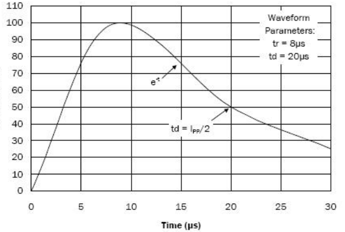
Fig.2 Pulse Waveform
